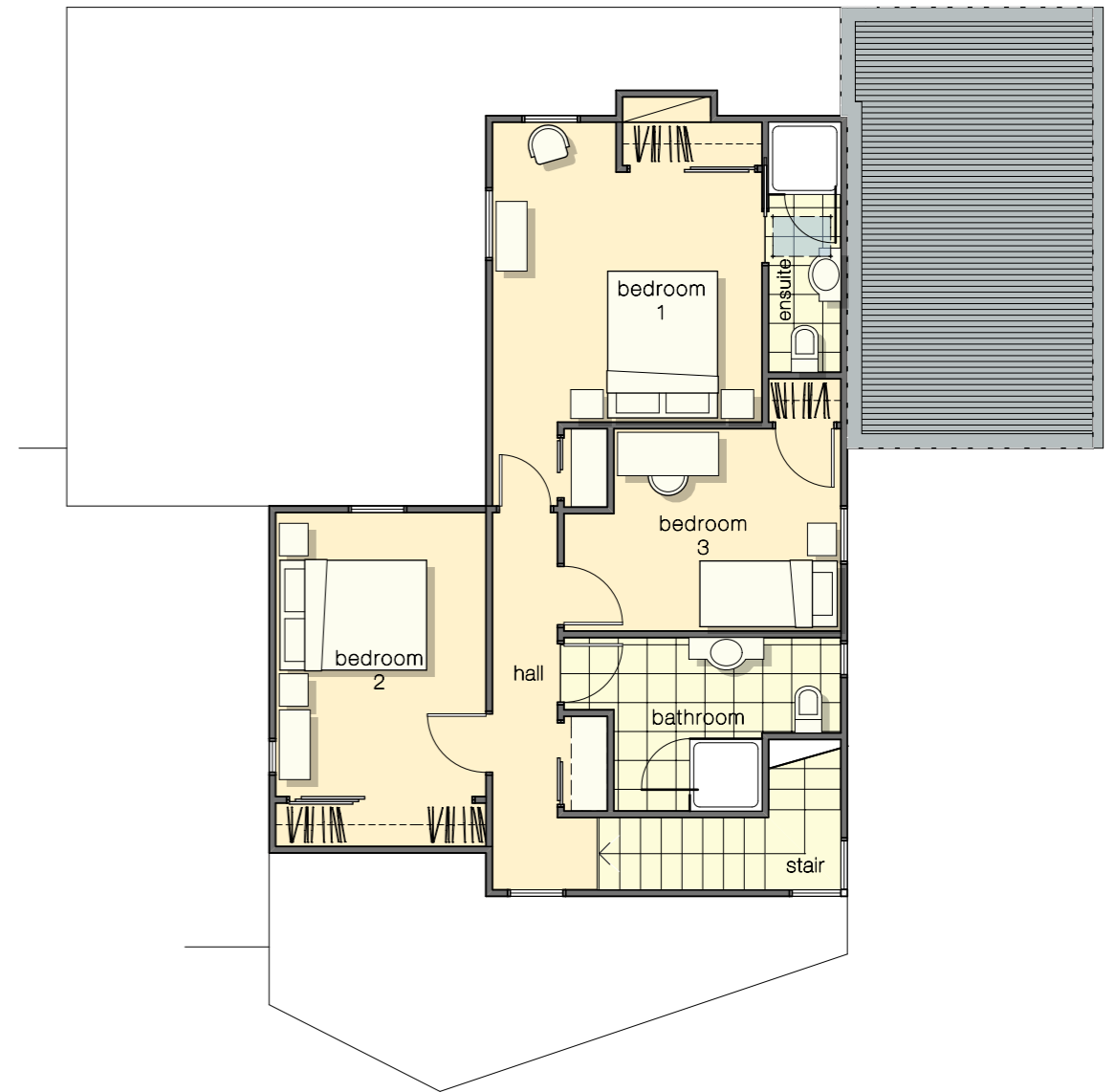
first floor 68.7 M 2
